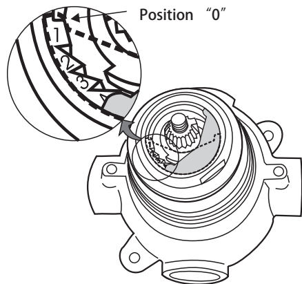
Figure 10. Setting the blend control
