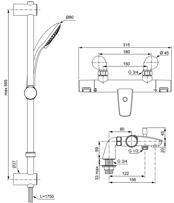
Bath/Shower Thermostat with shower bar and handspray chrome A7698AA
